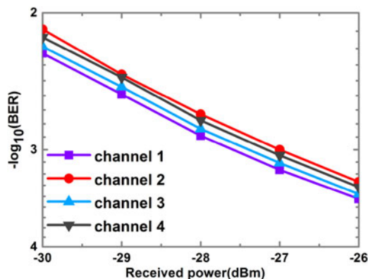
Fig. 8. BER performance versus received power after 160-km SMF transmission for four channels.
